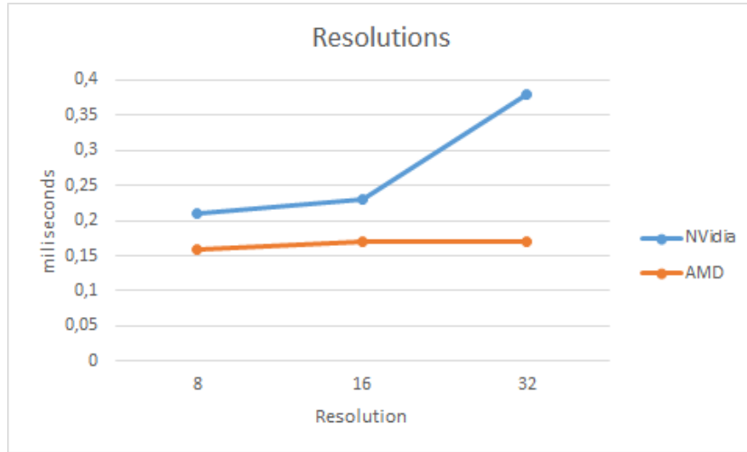
Figure 4.5: Rendering times for different per-face resolutions.
